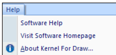
Figure 3.3: Help Menu
