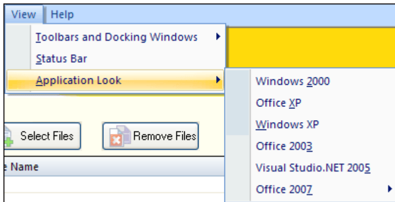
Figure 3.2: View Menu
